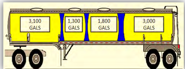
Fuel Trailer with bulkheads can carry different grades of fuel
