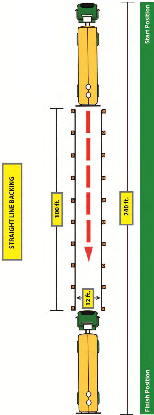
Figure 12.1 Straight Line Backing
