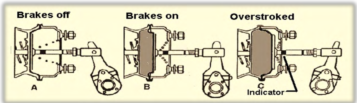
Figure 11.1 - Air Brake Adjustment
