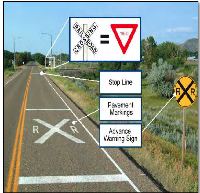
Figure 2.14 Railroad Crossing Signs
